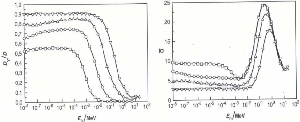
Figure 4(a). The ratio ( D_{\gamma}/D ) of absorbed dose contributed by photons D_{\gamma} to the total, D versus neutron energy for neutrons incident on phantoms of different size. Key: \square -Mouse; O -rat; \Delta - H^*(10) [value at 10mm in the ICRU sphere]; \nabla -weighted mean value in the ADAM phantom.
