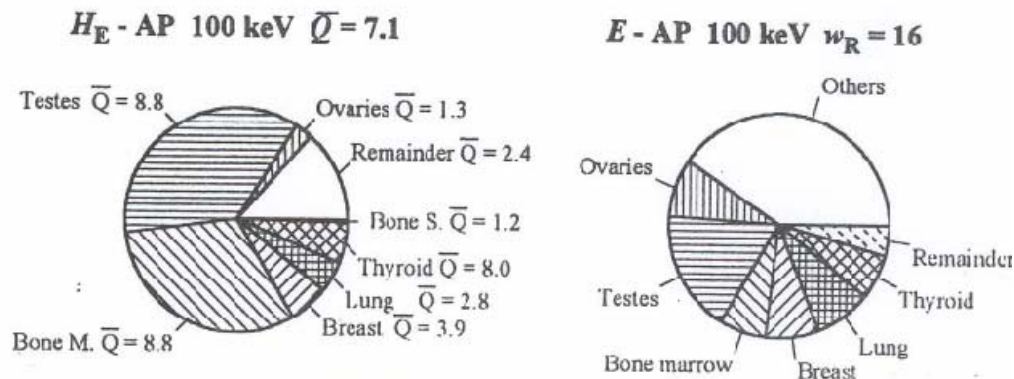
Figure 1. Relative contributions of specific organs to Effective Dose Equivalent, H_E , and to Effective Dose, ( E ), for 100 keV incident neutrons in AP irradiation geometry on an adult human computational model (mean of values calculated in ADAM and EVA). ICRP Publication 74 (fig.49)
