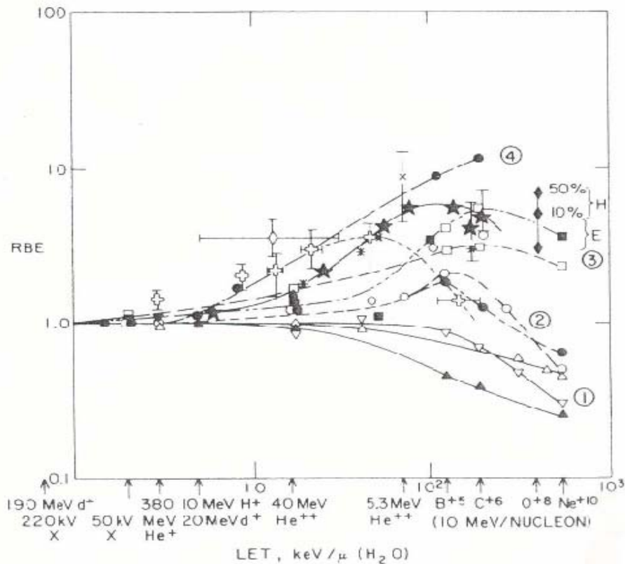
Figure 2. Experimental curves of RBE versus LET. Mammalian cells are indicated by the symbols * and □ (BNL 50073, 1967)
