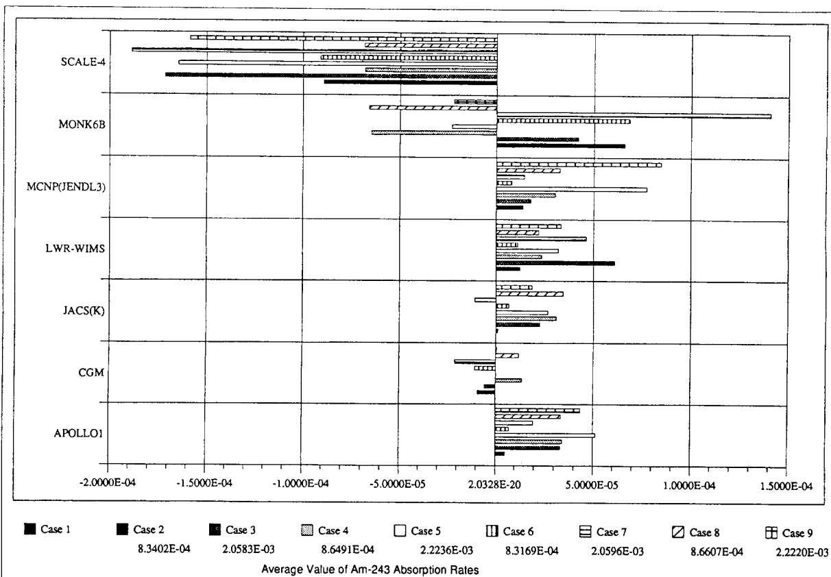
Fig. A3.3 Difference of Am-243 Absorption Rate from Average
