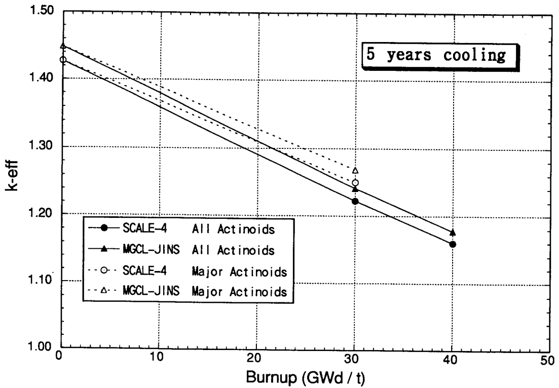
Fig. 2 Multiplication Factors ( k_{\text{eff}} ) with Burnup; Dependence on group constants (without fission product). Major Actinoids: U-234, 235, 236, 238, Pu-239, 240, 241 All Actinoids: Major Actinoids + Np-237, Pu-238, 242, Am-241
