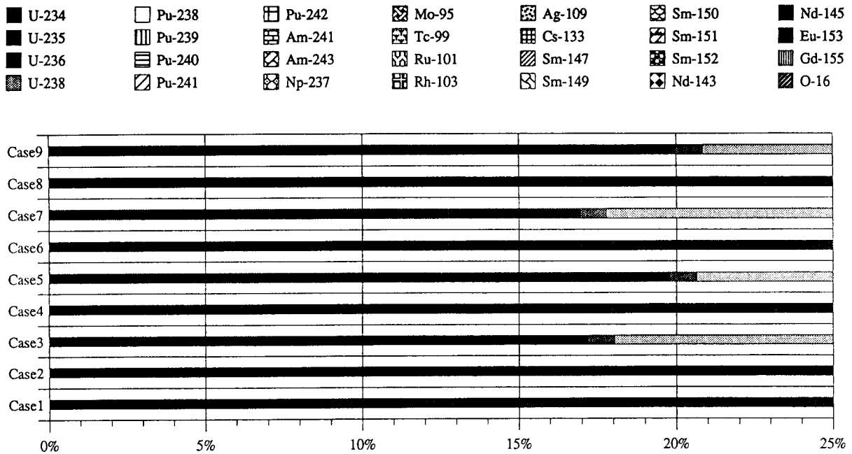
Fig. 4.19 Absorption-Rate of Each Nuclide (Enlarged)
