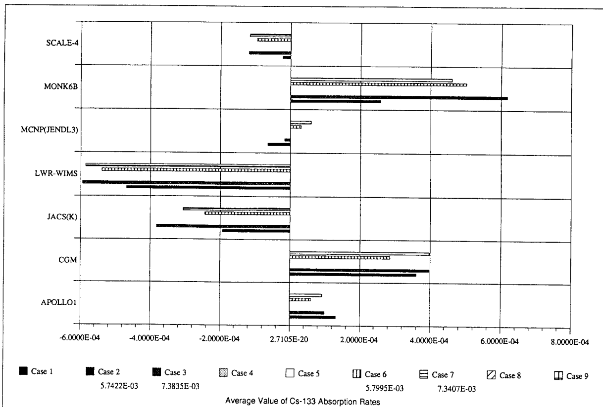
Fig. A3.4 Difference of Cs-133 Absorption Rate from Average
