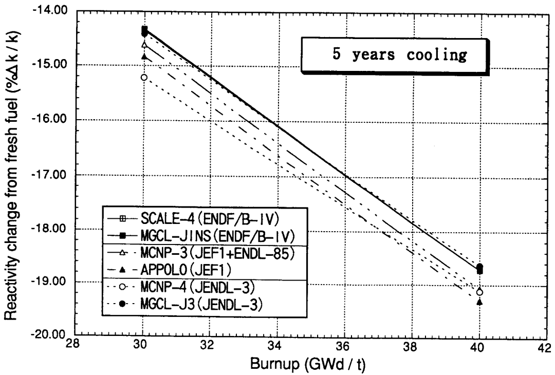
Fig. 4 Reactivity Changes from Fresh Fuel with Burnup; Dependence on evaluated nuclear data libraries. (without fission product, including all 12 actinoids)
