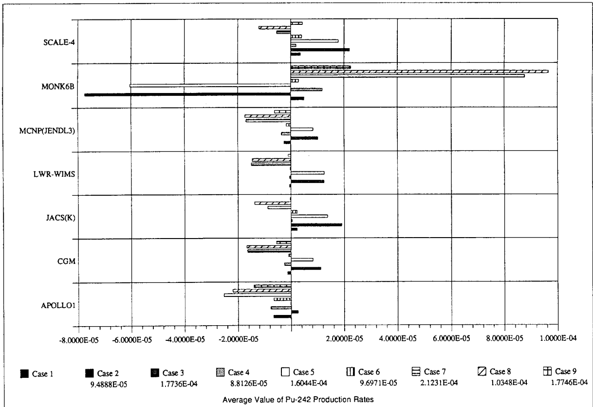
Fig. A3.36 Difference of Pu-242 Production Rate from Average
