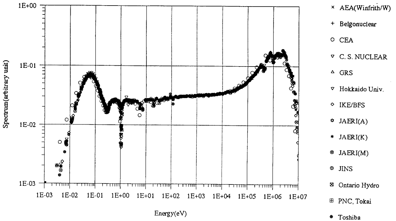
Fig. 4.9 CASE 7 Spectrum in Fuel (40GWd/t, 5yr, selected F.P.)
