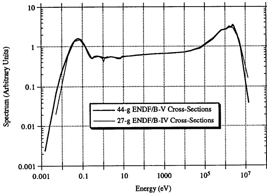
Fig. 4 Case 7 Flux in Reflector (40 GWD/t, 5y, Major FPs)
