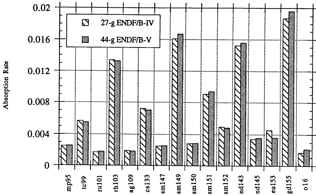
Fig. 8 Absorption in FPs, Case 7 (40 GWD/t, 5y Cooling Time, Major FPs)
