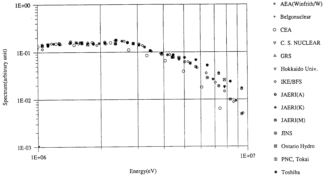
Fig. 4.15 CASE 1 Spectrum in Fuel (From 1 MeV to 10 MeV)
