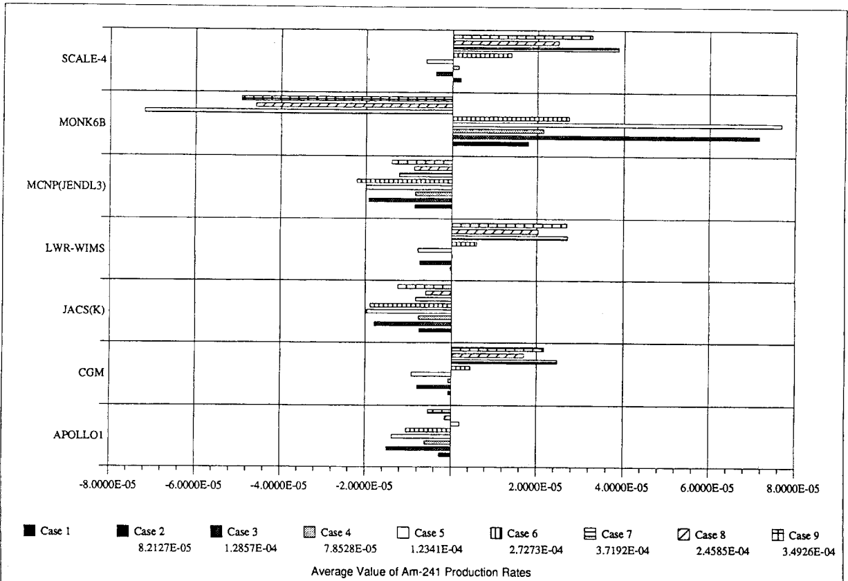
Fig. A3.29 Difference of Am-241 Production Rate from Average
