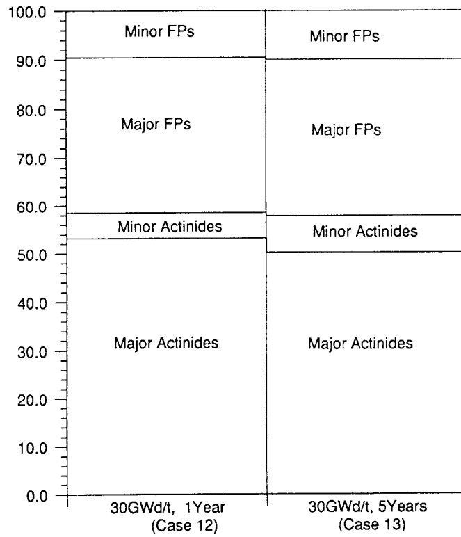
Fig. 4.6 Contributions to Reactivity Loss
