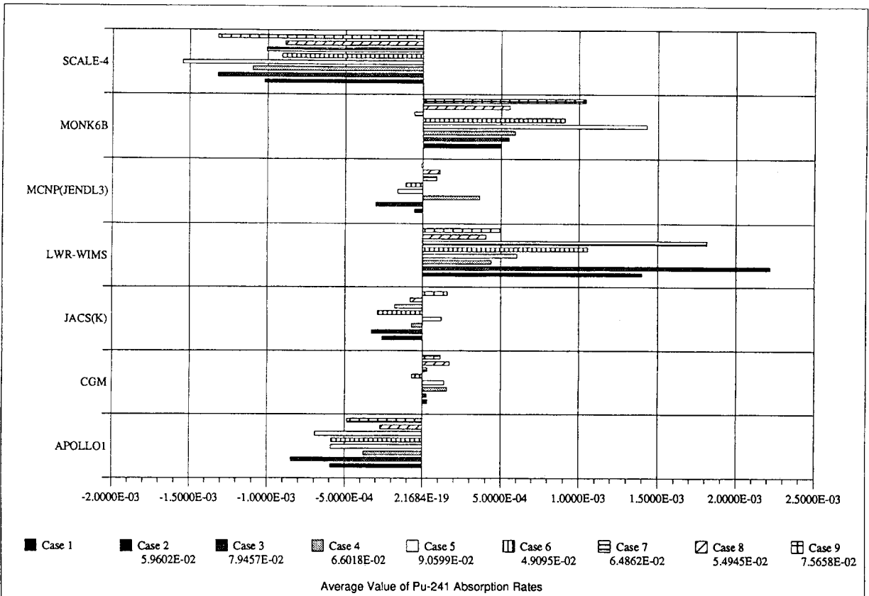
Fig. A3.15 Difference of Pu-241 Absorption Rate from Average
