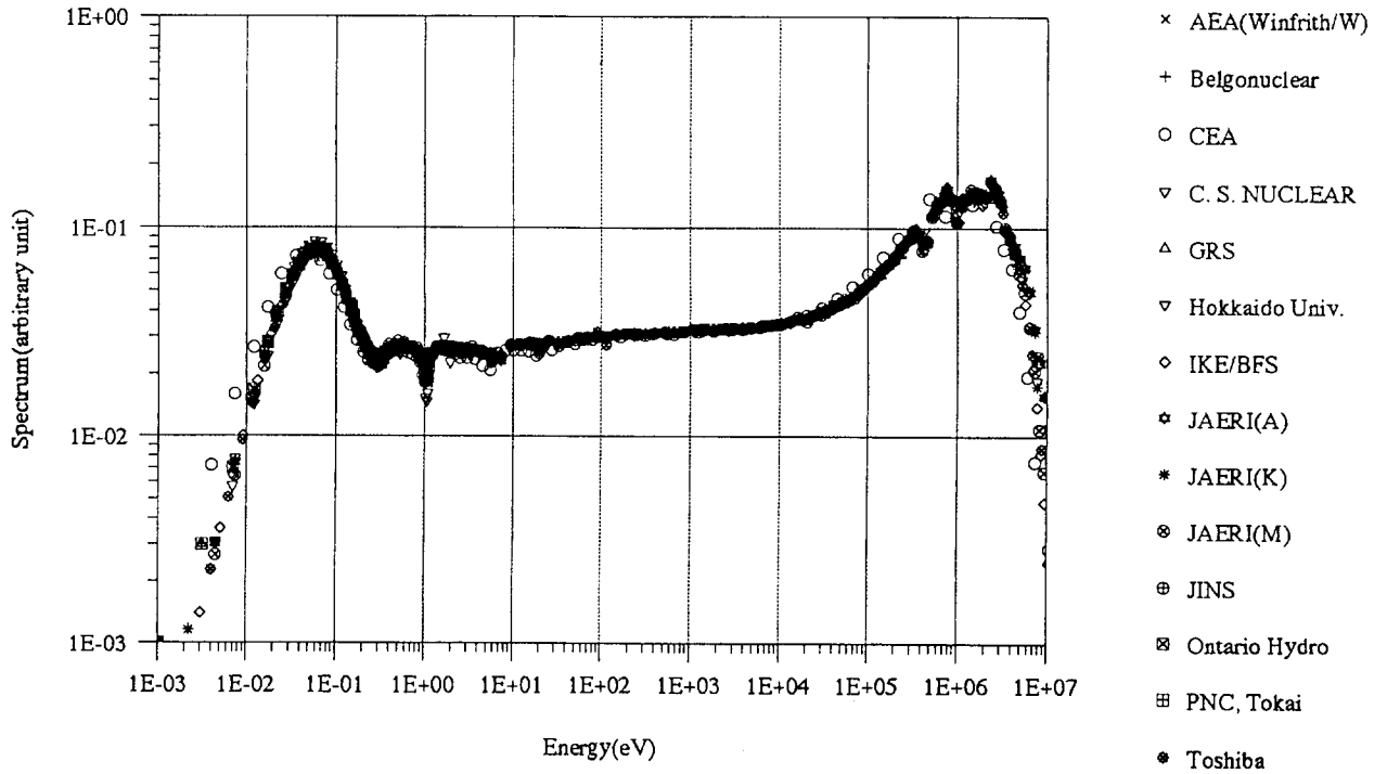
Fig. 4.12 CASE 7 Spectrum in Reflector (40Gwd/t, 5yr, selected F.P.)
