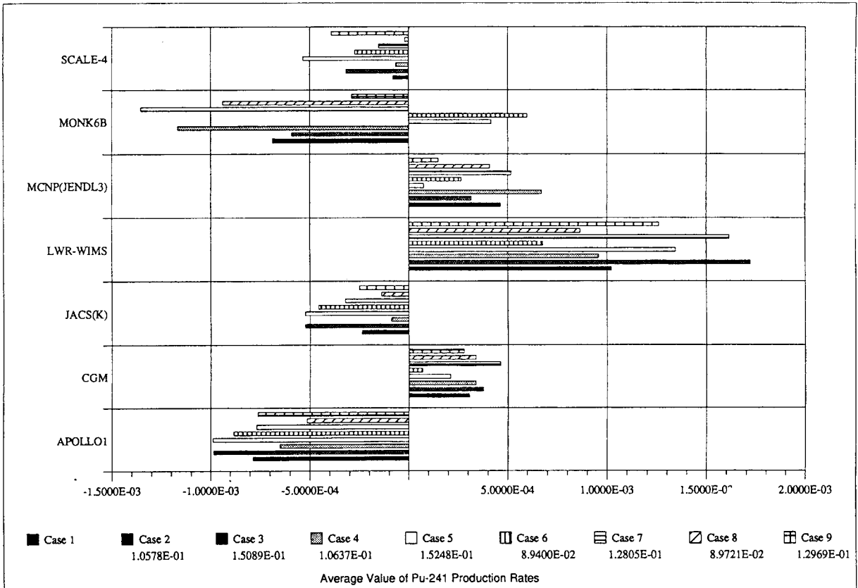
Fig. A3.35 Difference of Pu-241 Production Rate from Average
