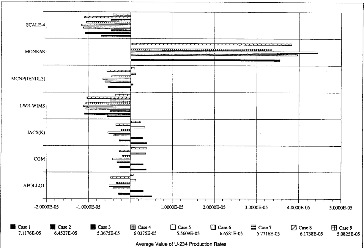
Fig. A3.37 Difference of U-234 Production Rate from Average
