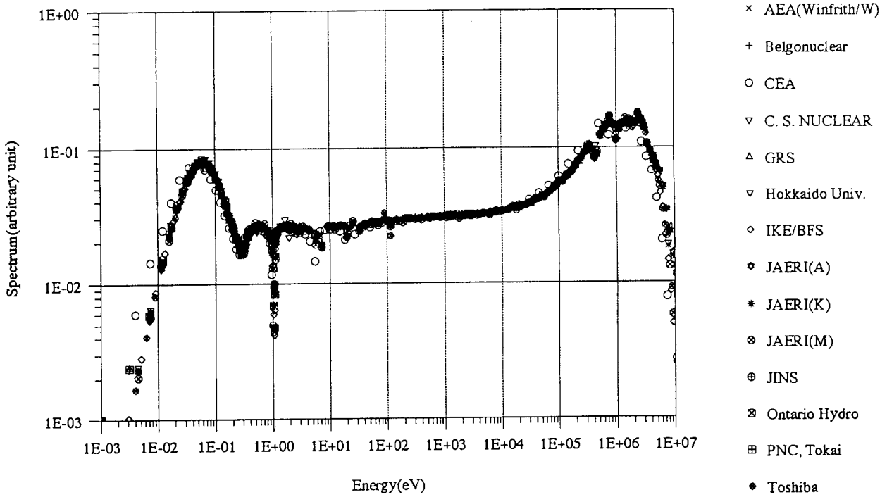
Fig. 4.10 CASE 9 Spectrum in Fuel (40Gwd/t, 5yr, no F.P.)
