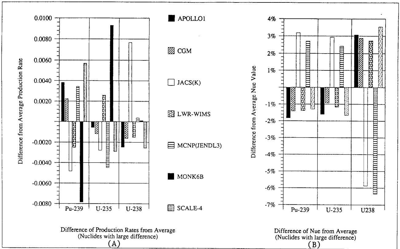
Fig. 4.17 Nuclides with Large Differences of Production Rates and \nu Values (Case 7)
