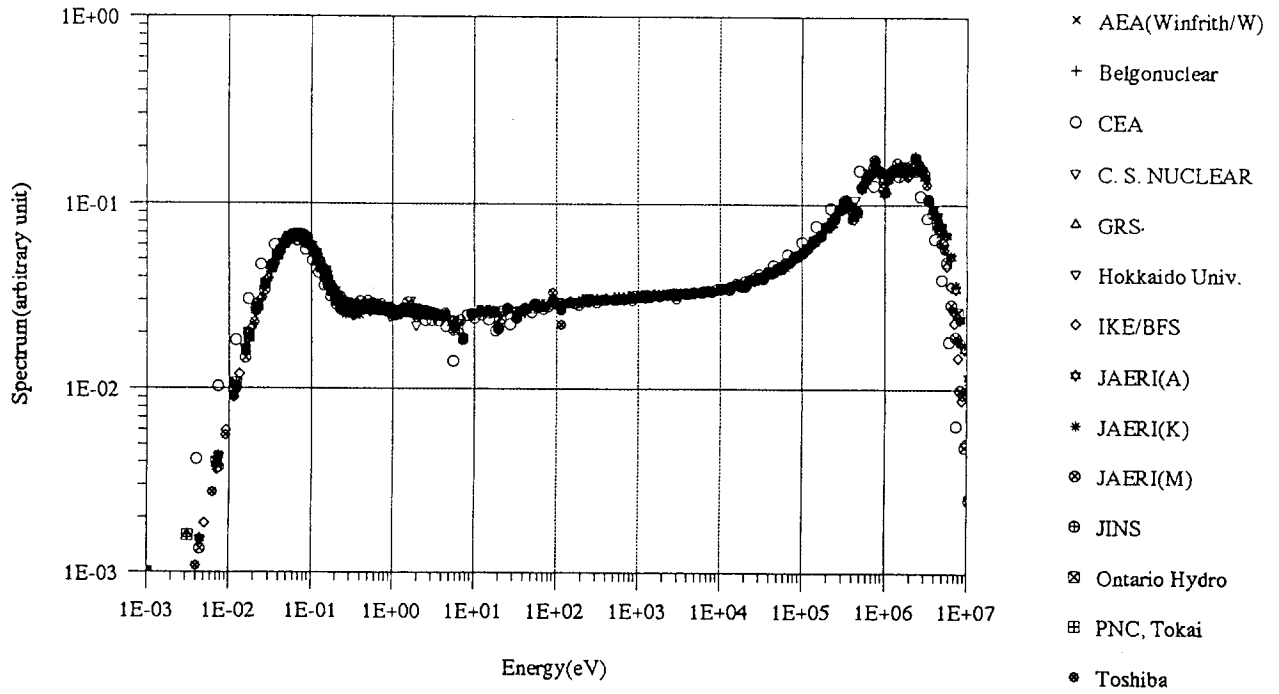
Fig. 4.8 CASE 1 Spectrum in Fuel (Fresh Fuel)
