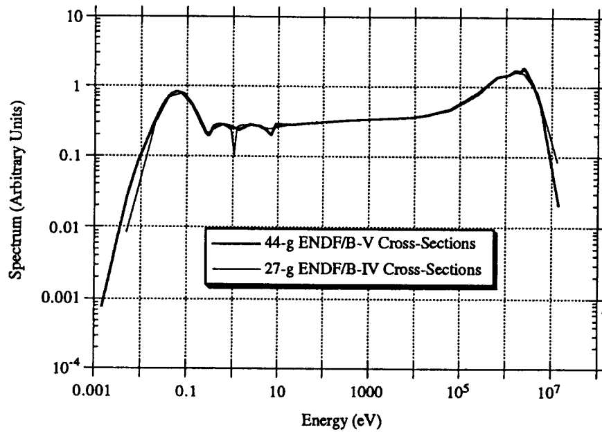
Fig. 5 Case 9 Flux in Fuel (40 GWD/t, 5y, No FPs)
