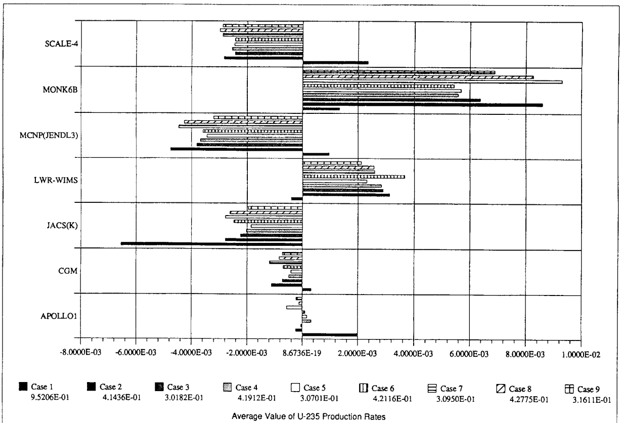
Fig. A3.38 Difference of U-235 Production Rate from Average
