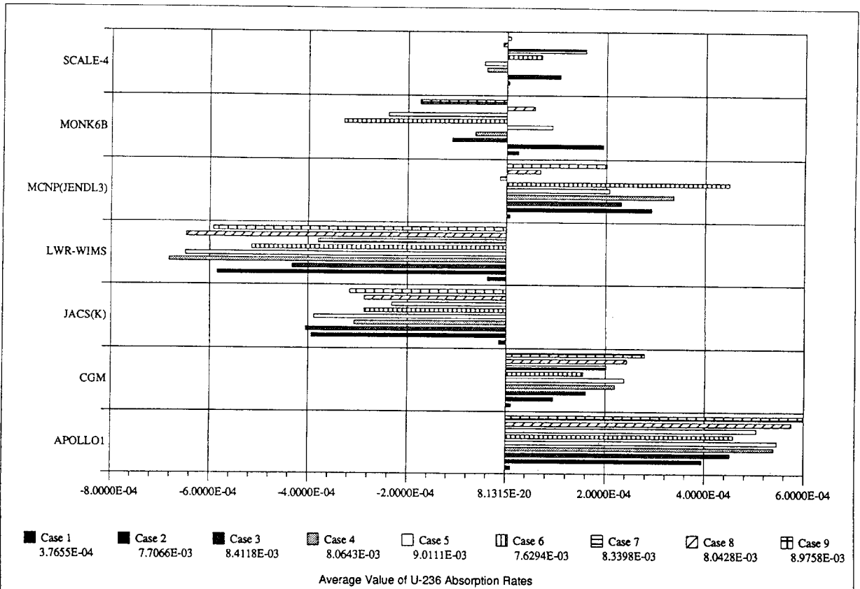
Fig. A3.27 Difference of U-236 Absorption Rate from Average
