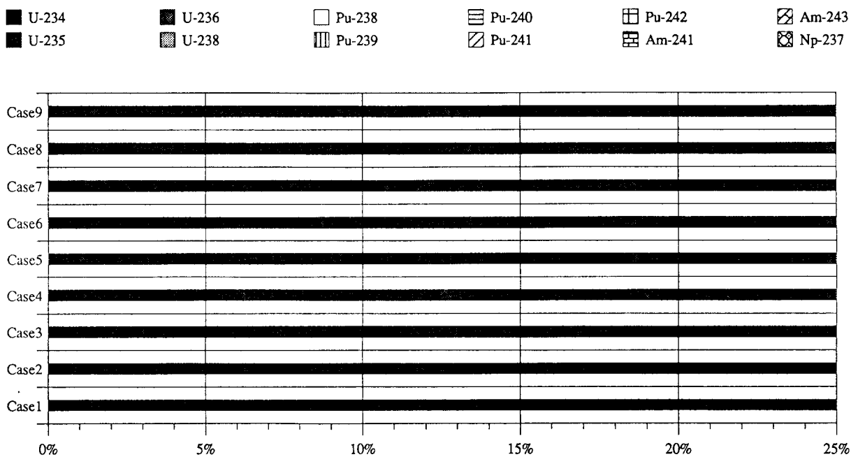
Fig. 4.21 Production-Rate of Each Nuclide (Enlarged)
