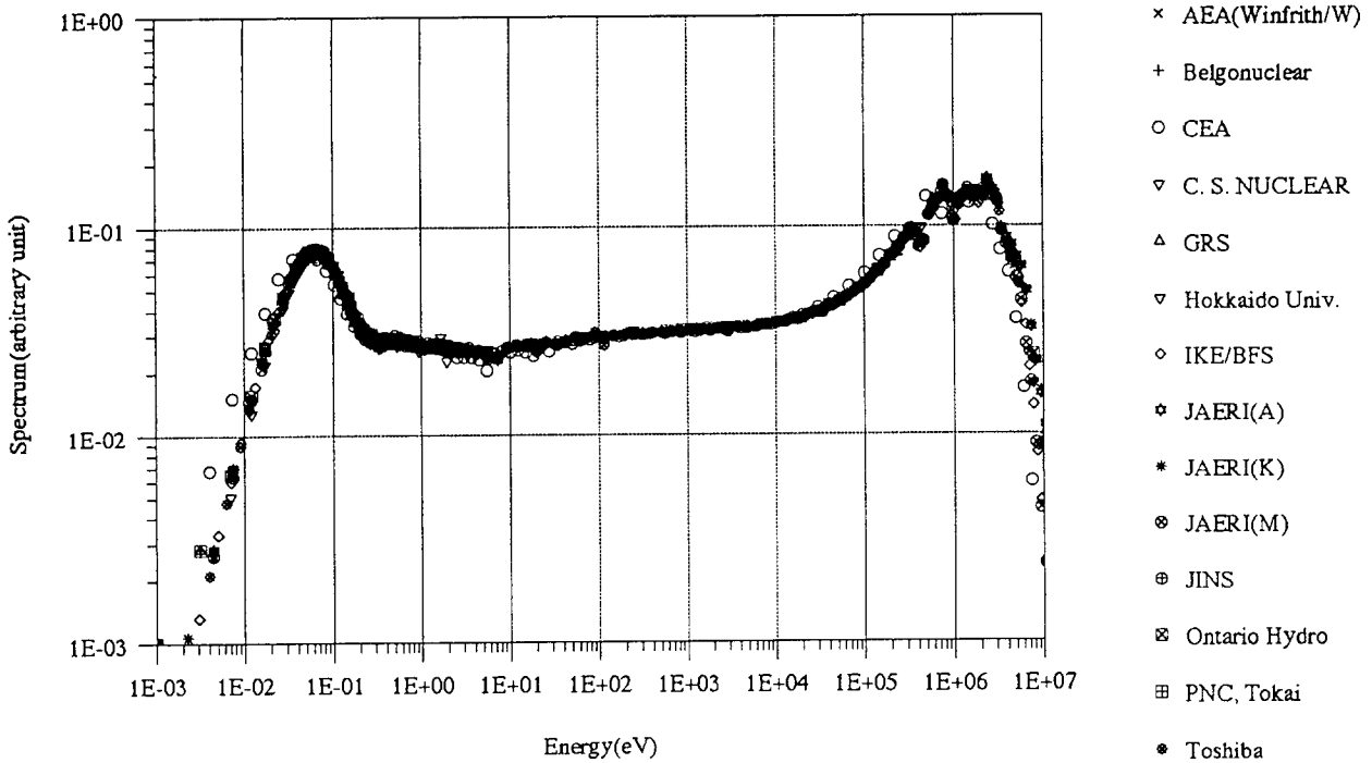
Fig. 4.11 CASE 1 Spectrum in Reflector (Fresh Fuel)
