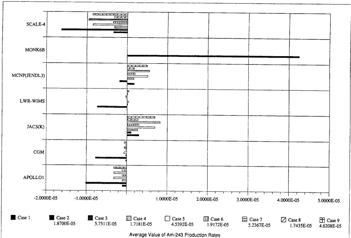
Fig. A3.30 Difference of Am-243 Production Rate from Average
