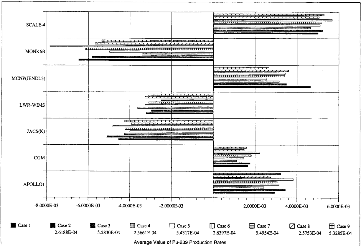
Fig. A3.33 Difference of Pu-239 Production Rate from Average
