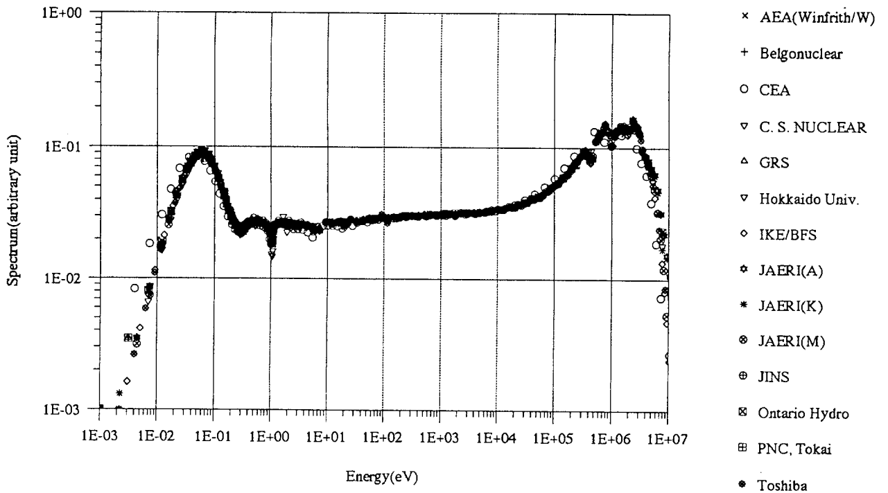
Fig. 4.13 CASE 9 Spectrum in Reflector (40Gwd/t, 5yr, no F.P.)
