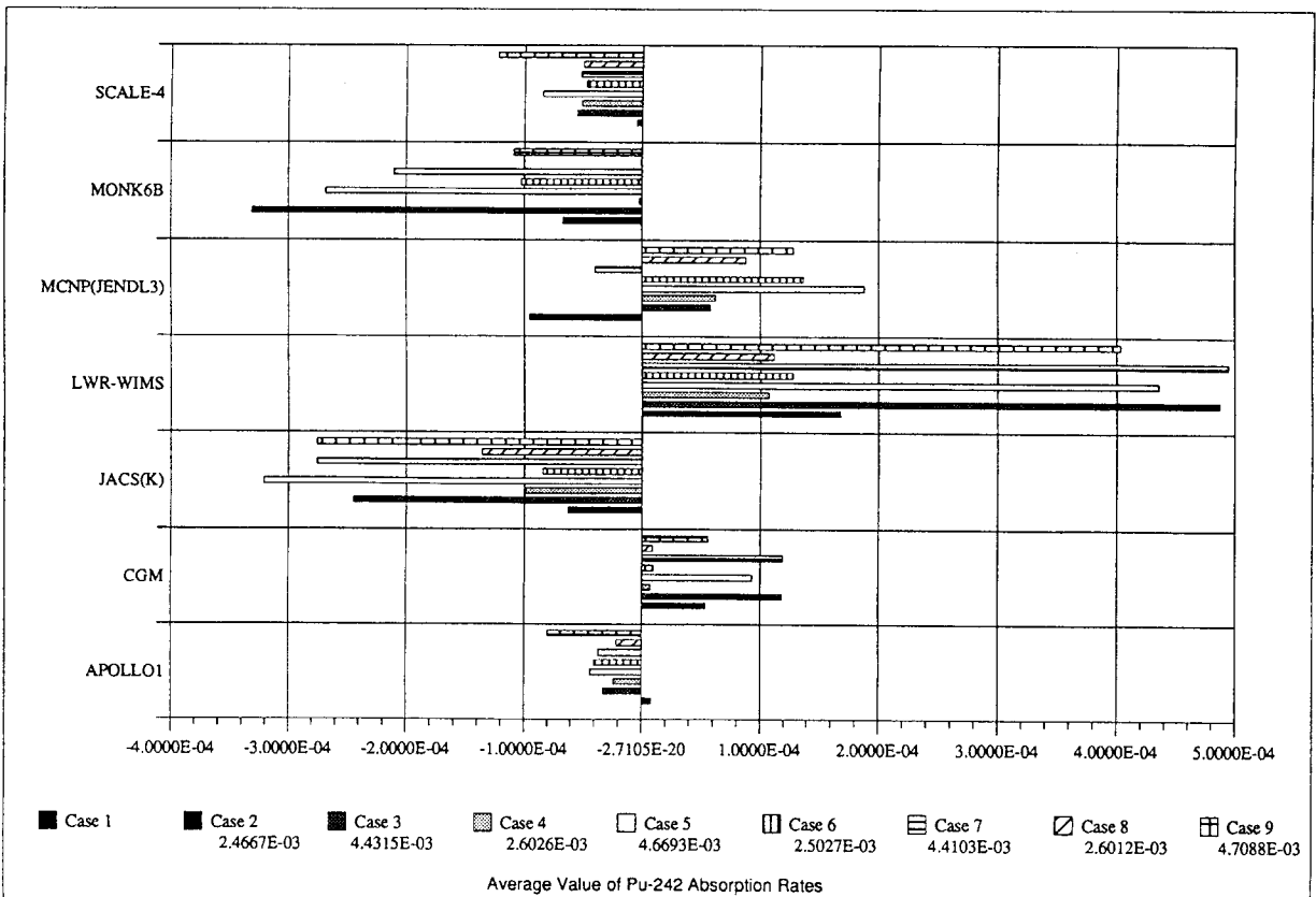
Fig. A3.16 Difference of Pu-242 Absorption Rate from Average
