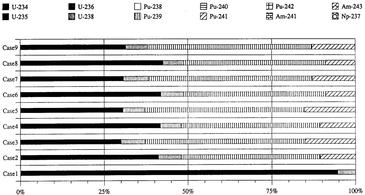
Fig. 4.20 Production-Rate of Each Nuclide (Example)
