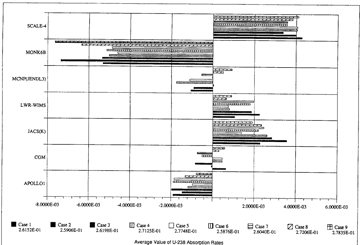
Fig. A3.28 Difference of U-238 Absorption Rate from Average
