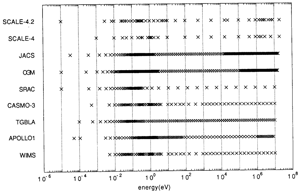
Fig. 4.7 Upper Energy Boundaries
