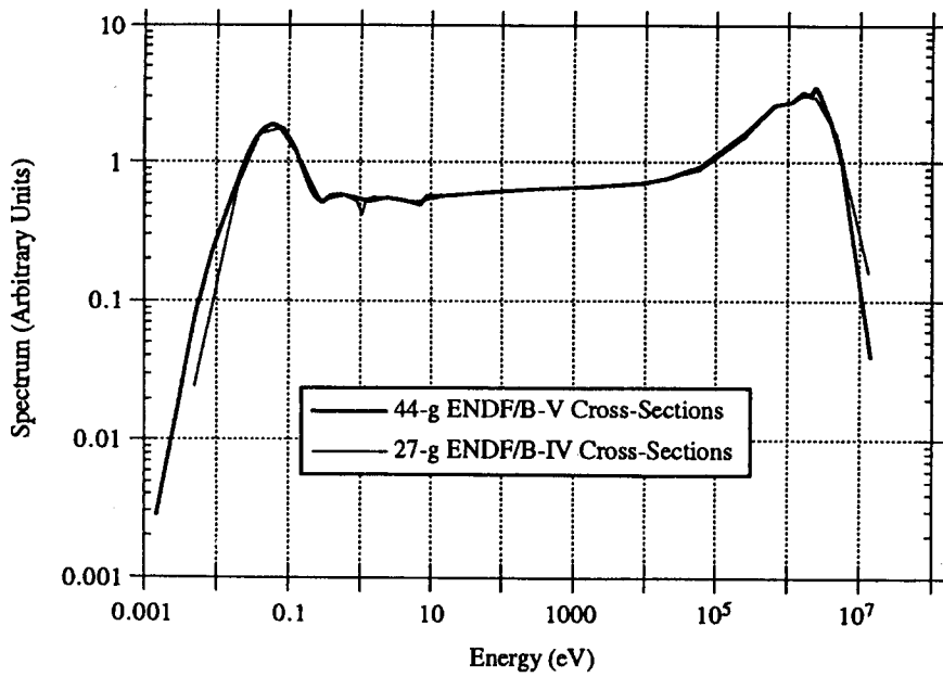
Fig. 6 Case 9 Flux in Reflector (40 GWD/t, 5y, No FPs)
