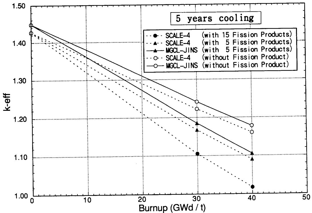
Fig. 1 Multiplication Factors (k-eff) with Burnup; Dependence on group constants and fission products (including all 12 actinoids).
