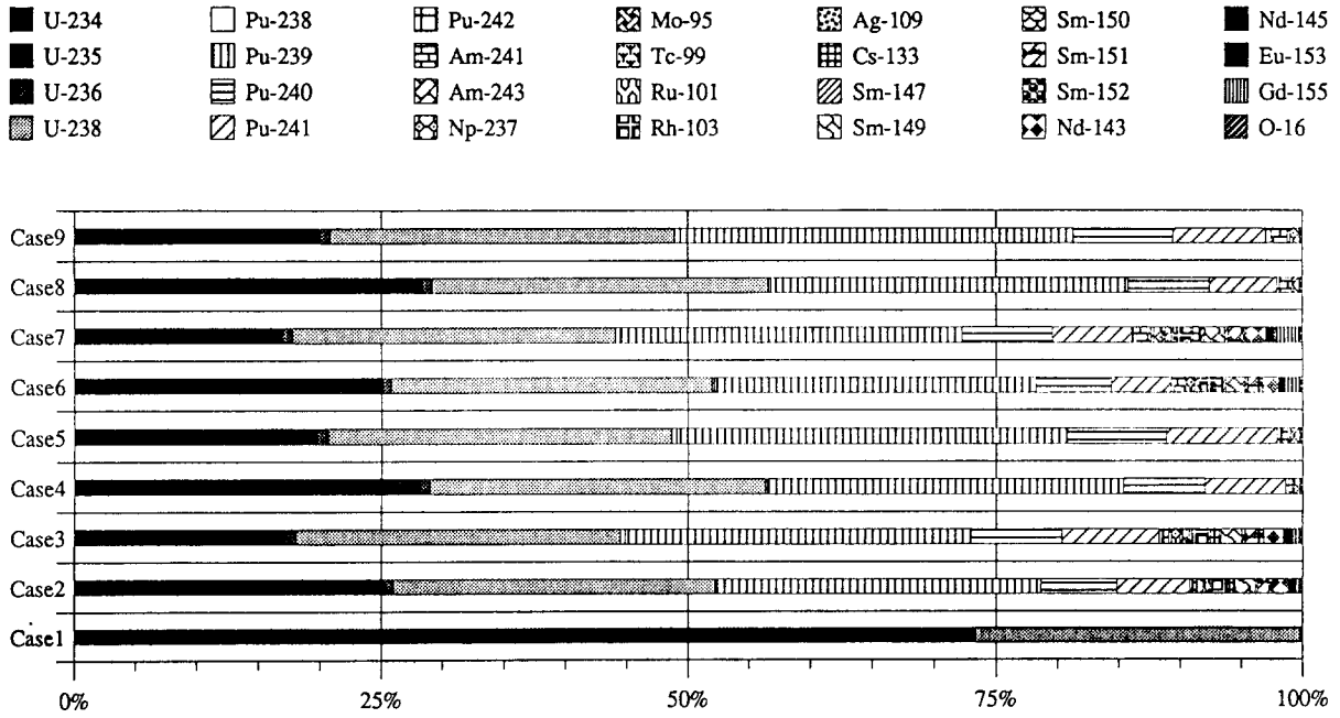
Fig. 4.18 Absorption-Rate of Each Nuclide (Example)
