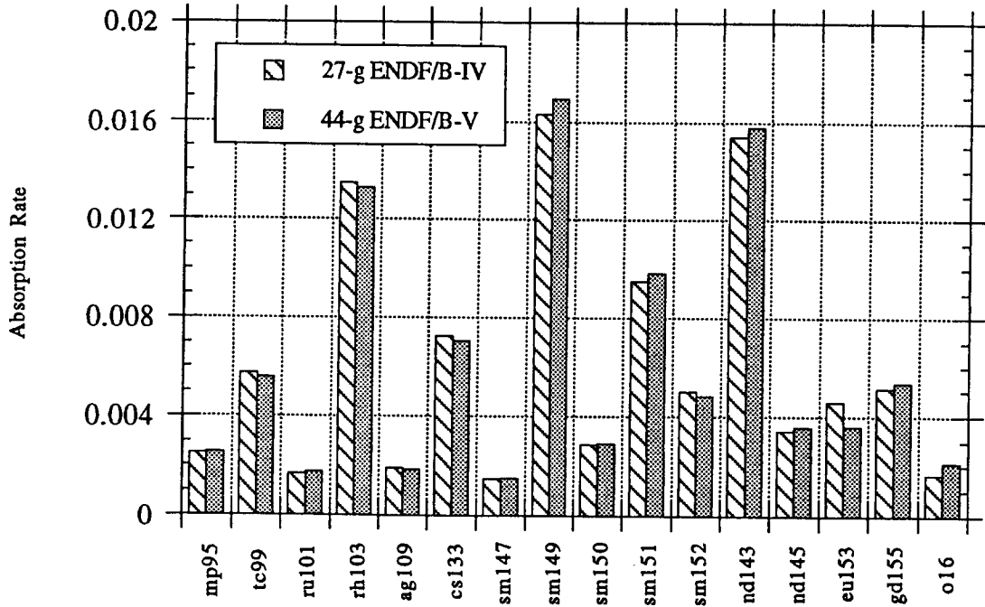
Fig. 7 Absorption in FPs, Case 3 (40 GWD/t, 1y Cooling Time, Major FPs)
