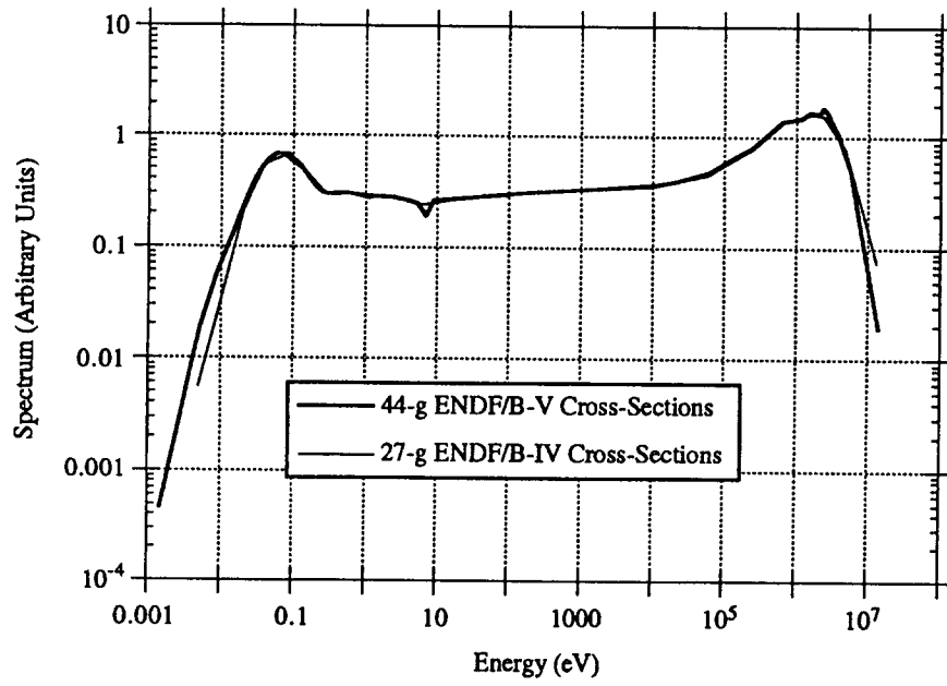
Fig. 1 Case 1 Flux in Fuel (Fresh Fuel)
