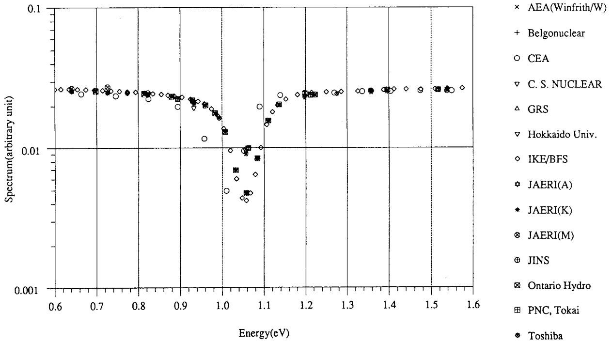
Fig. 4.14 CASE 9 Spectrum in Fuel (From 0.6 to 1.4 eV.)
