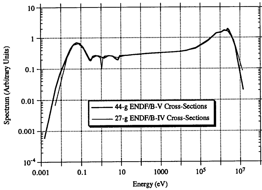
Fig. 3 Case 7 Flux in Fuel (40 GWD/t, 5y, Major FPs)
