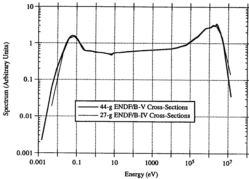
Fig. 2 Case 1 Flux in Reflector (Fresh Fuel)
