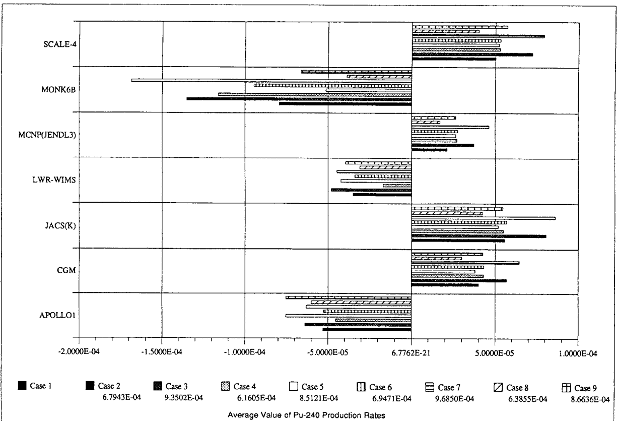
Fig. A3.34 Difference of Pu-240 Production Rate from Average
